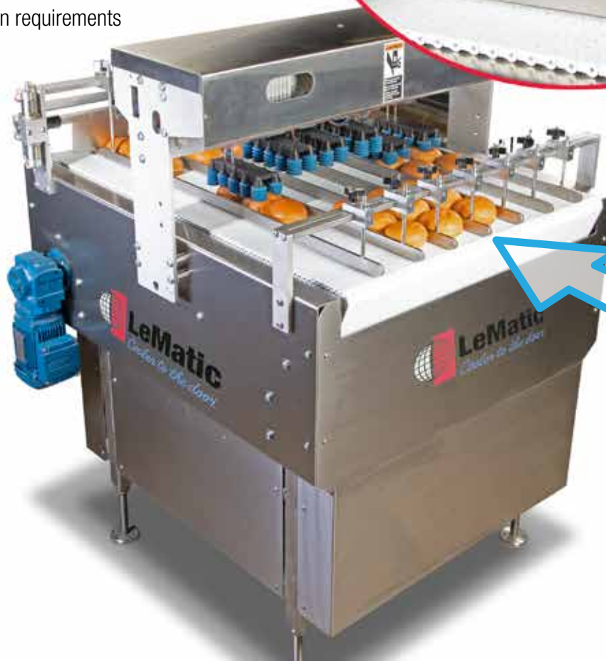
Product Flow
